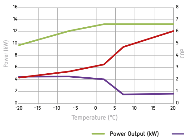
Winchester Performance at 35°C Outlet Temperature
