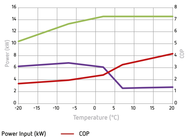
Winchester Performance at 55°C Outlet Temperature
